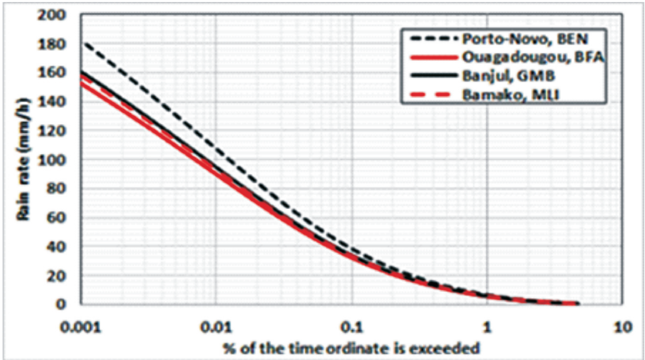
Figure 3: CCDF of the rainfall rates (mm/h) for Benin, Burkina Faso, Gambia, and Mali.
